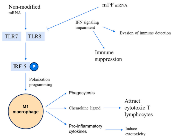
Fig. 3. Schematic representation of the potential effects of 100 % modified vs. unmodified mRNA vaccines on Toll-like receptors (TLRs). In a similar fashion to suppression of innate immune functions observed with RLRs, suppression of TLRs could also negatively impact proper anti-cancer surveillance by impacting induction of M1 macrophage polarization.
