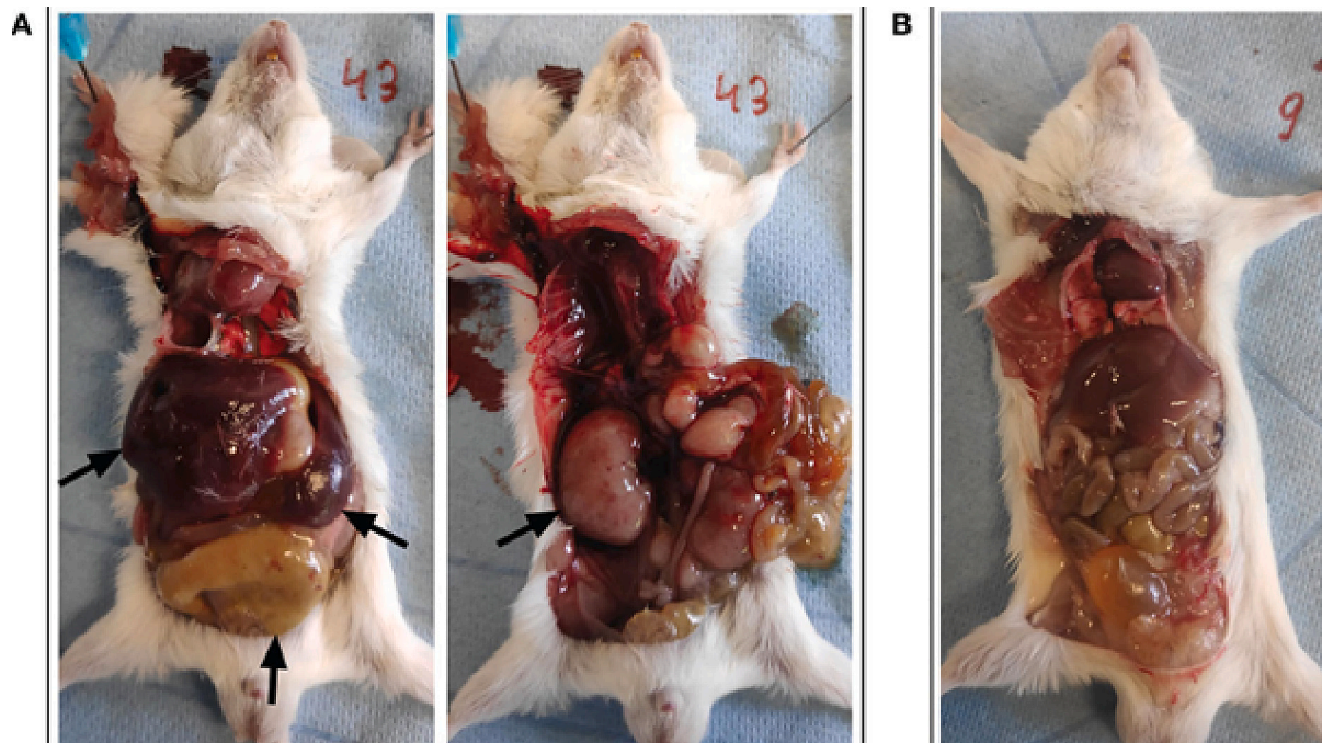
Fig. 7. Organs were examined during a necropsy after a spontaneous death, which revealed lymphoid neoplasm two days after booster vaccination with BNT162b2. (A) At necropsy, several of the animal's primary organs, including the liver, kidneys, spleen, and intestines (black arrows), showed disproportionate hypertrophy. (B) A reference animal with a typical morphology. This is an open-access article distributed under the terms of the Creative Commons Attribution License (CC BY). The use, distribution, or reproduction in other forums is permitted, provided the original author(s) and the copyright owner(s) are credited and that the original publication in this journal is cited, in accordance with accepted academic practice. Source: [138].
